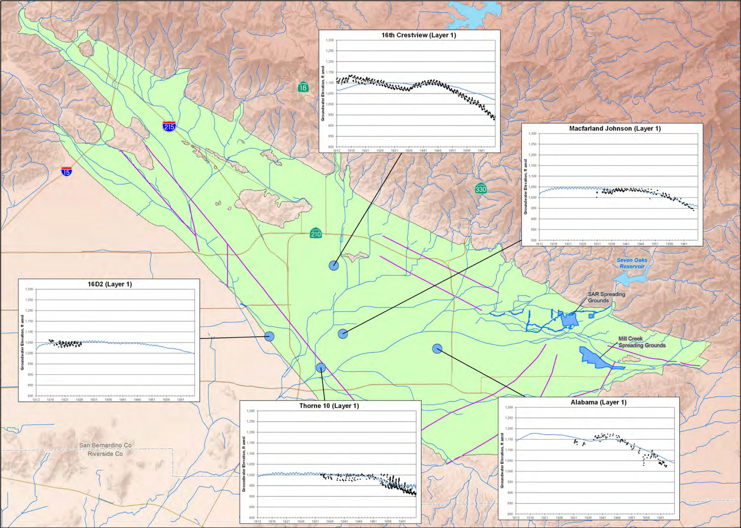
SELECTED HYDROGRAPHS IN THE SBBA MODEL AREA 1912-1965
