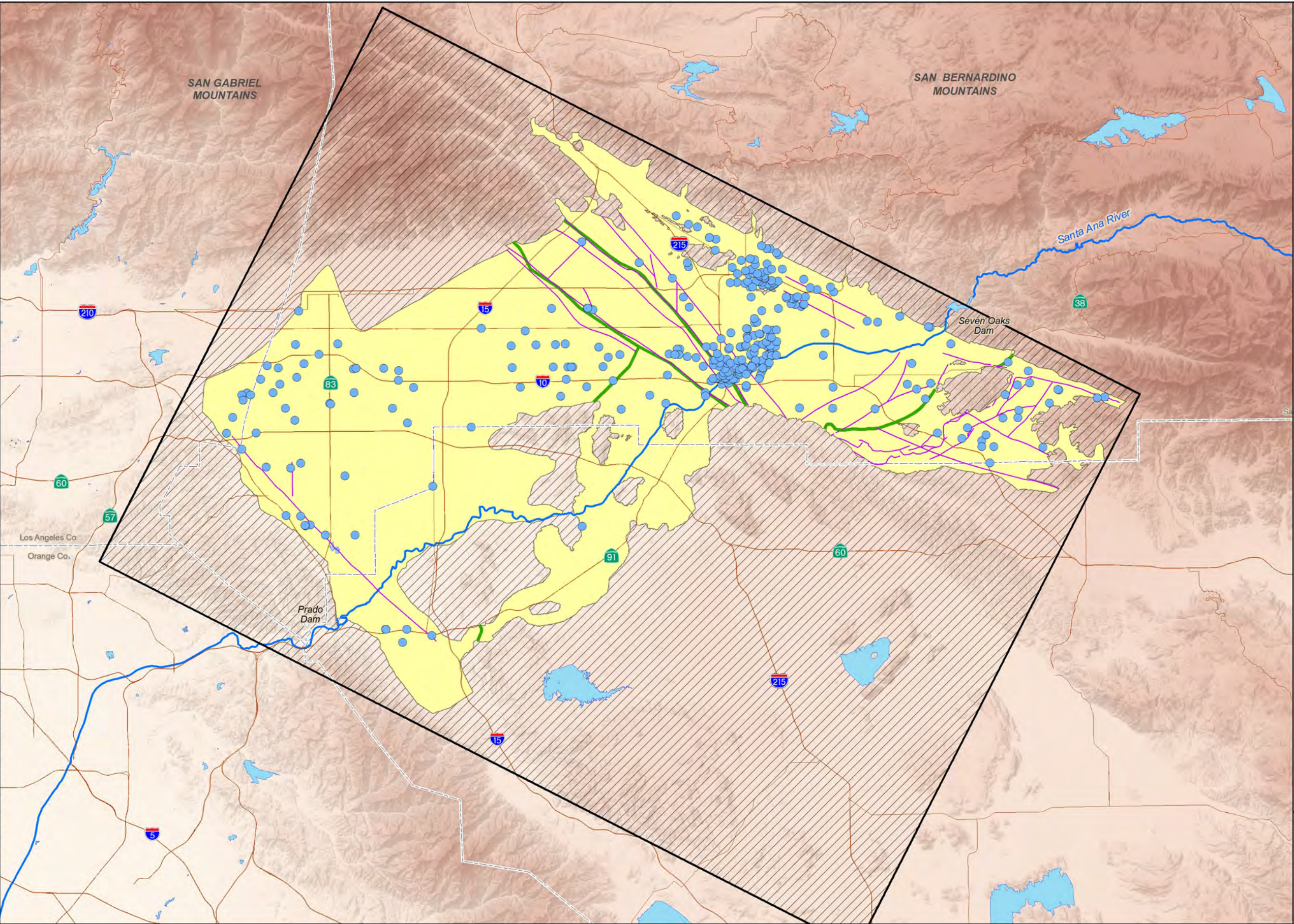
LOCATION OF WATER LEVEL TARGETS 1912-1965
